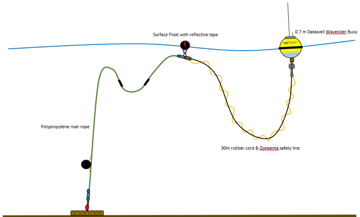
Deployed Wave Rider Buoy
