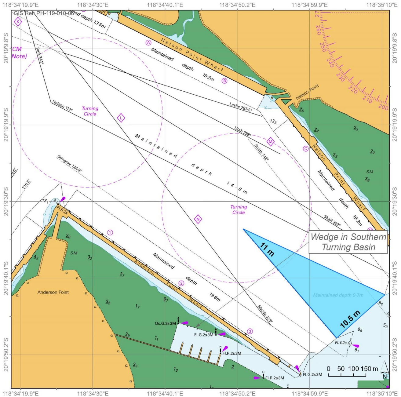
Figure 3. Southern Turning Basin Maintained Depth 10.6
