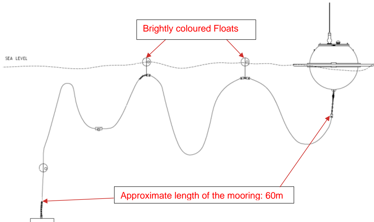
Mooring System Schematic for the Waverider Buoy
